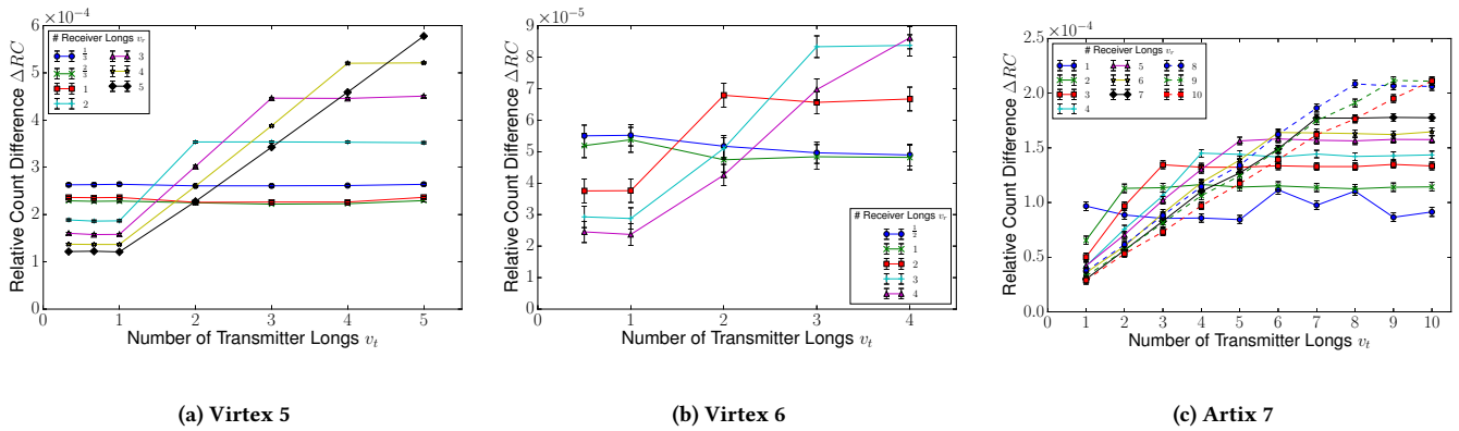
Figure 9: Relative frequency changes \Delta RC with 99% confidence intervals as a function of the transmitter and receiver lengths for different FPGA generations. The count difference is proportional to the overlap between the transmitter and the receiver.
