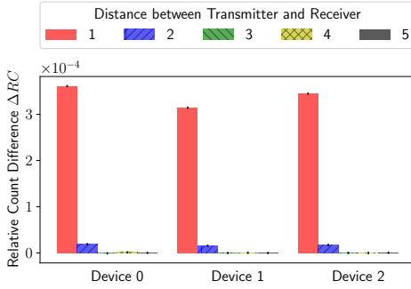
Figure 12: Effect of the transmitter-receiver distance. Long wires leak information up to two wires away. Distance is defined as in Figure 11.
